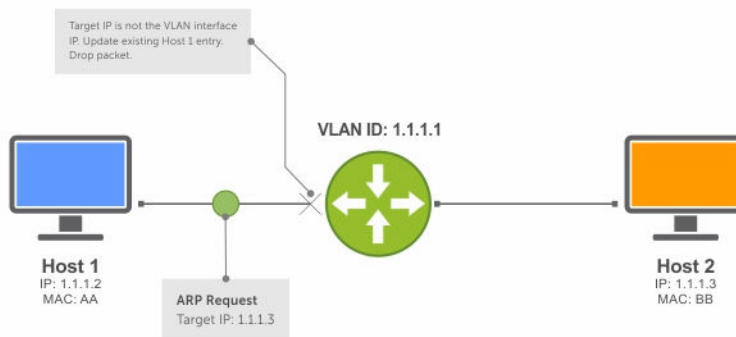
Figure 42. ARP Learning via ARP Request
